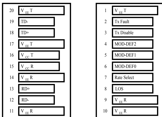
Bottom of Board (As Viewed through Top of Board)
